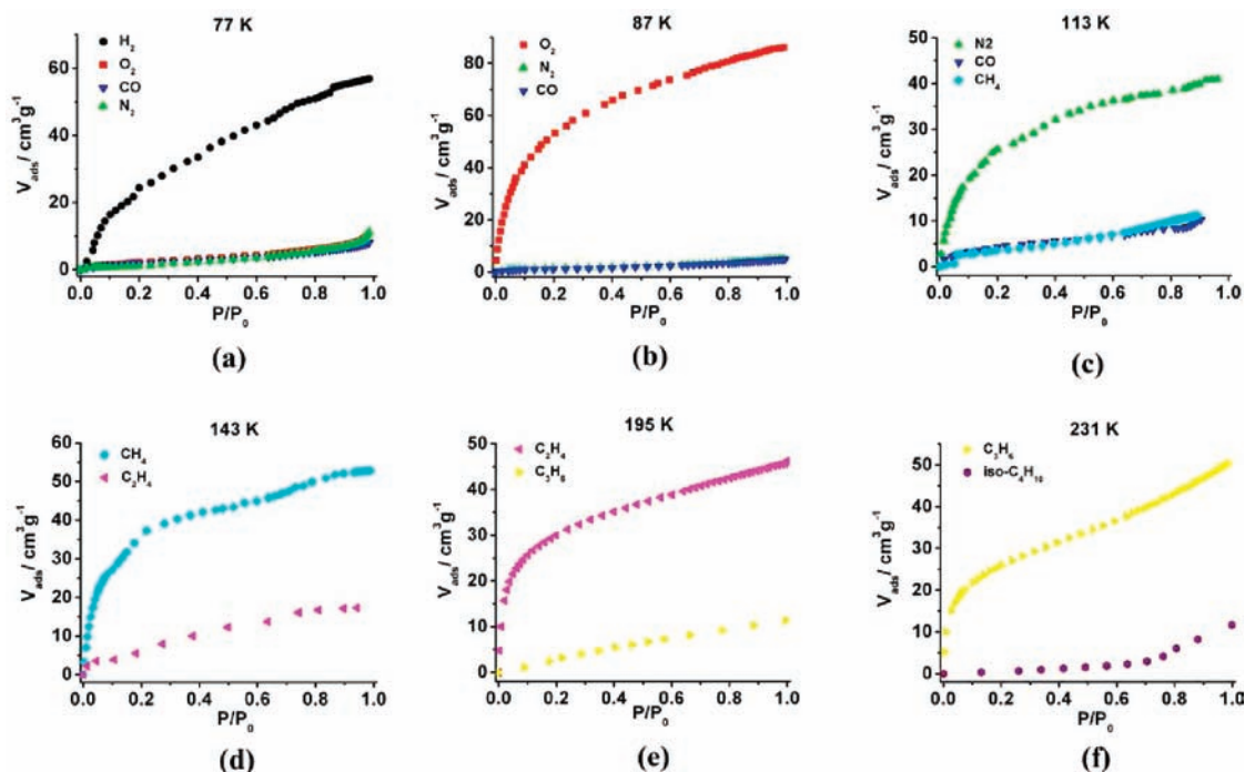
Figure 7. Gas adsorption isotherms of MAMS-2 at six different temperatures (note: P_0 represents a relative standard as specified in the Experimental Section).
